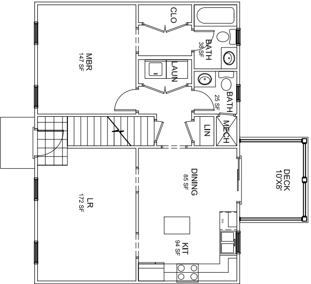
GROUND FLOOR - 792 SQ. FEET ( UNFINISHED)
